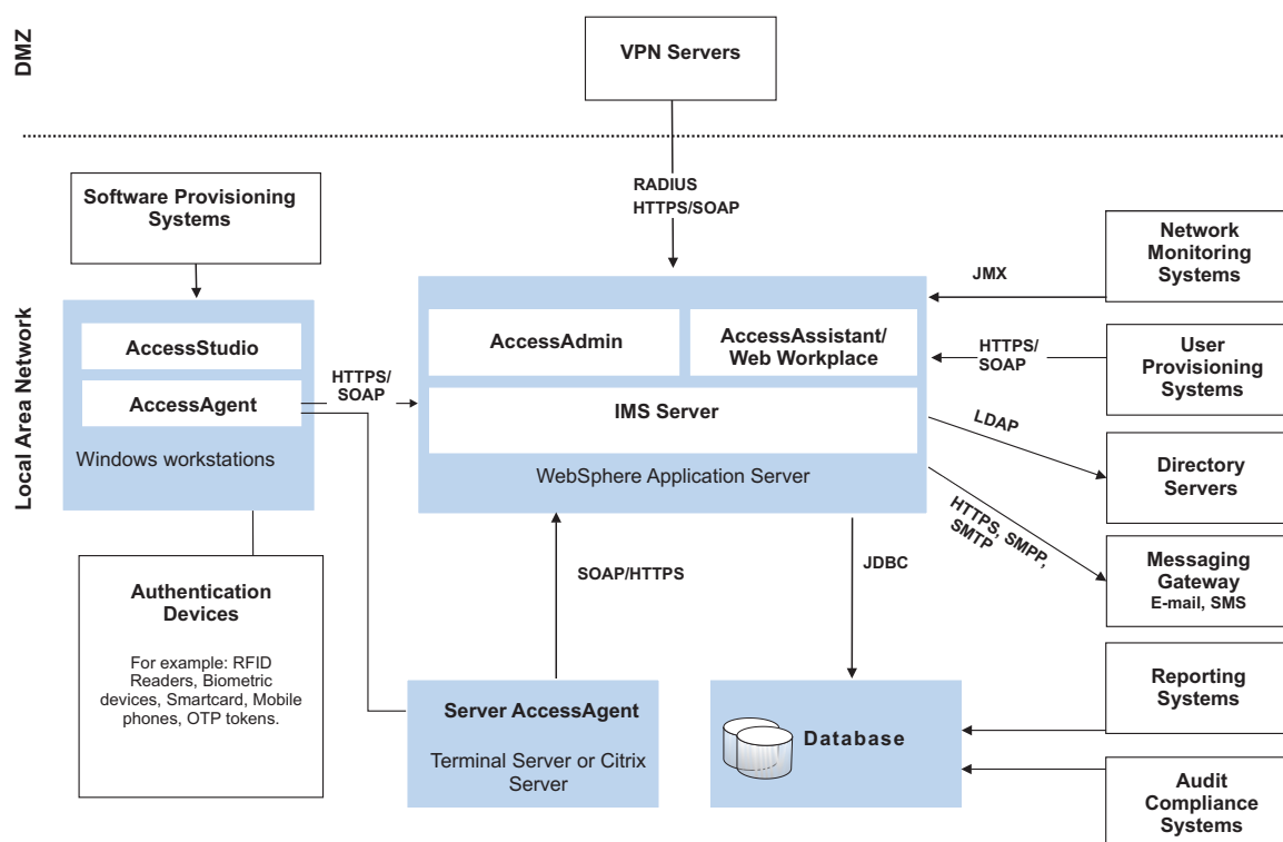
Figure 2. Overview of the IBM Security Access Manager for Enterprise Single Sign-On solution and integration with additional systems in an enterprise.
